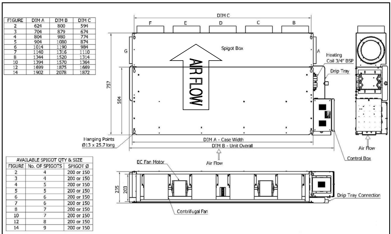
Diagram 2: Range of standard sizes with discharge plenum
