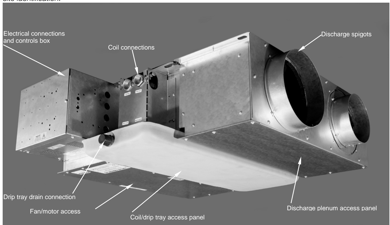
Diagram 1 - Series CRE Fig 3 LH connections with rectangular discharge plenum
